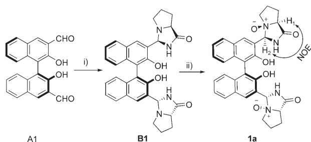
Scheme 1. Synthesis of the catalyst: i) L-prolinamide, ethanol, reflux; ii) m CPBA, CH 2 Cl 2 , –78 °C.
