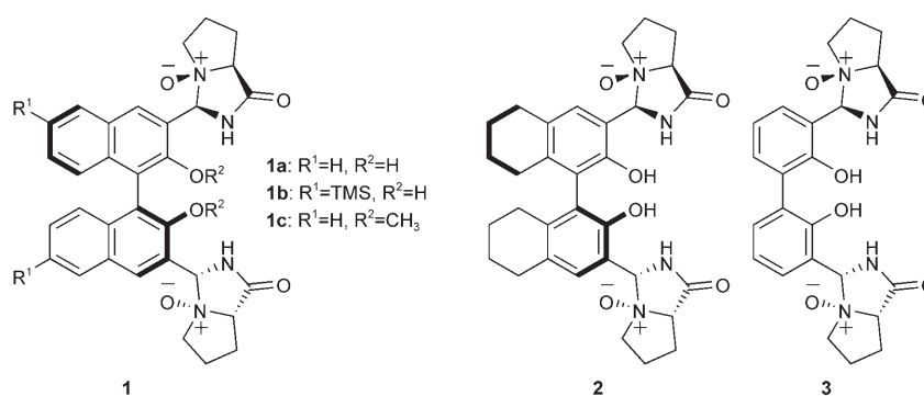
Figure 1. Catalysts used in this research.
